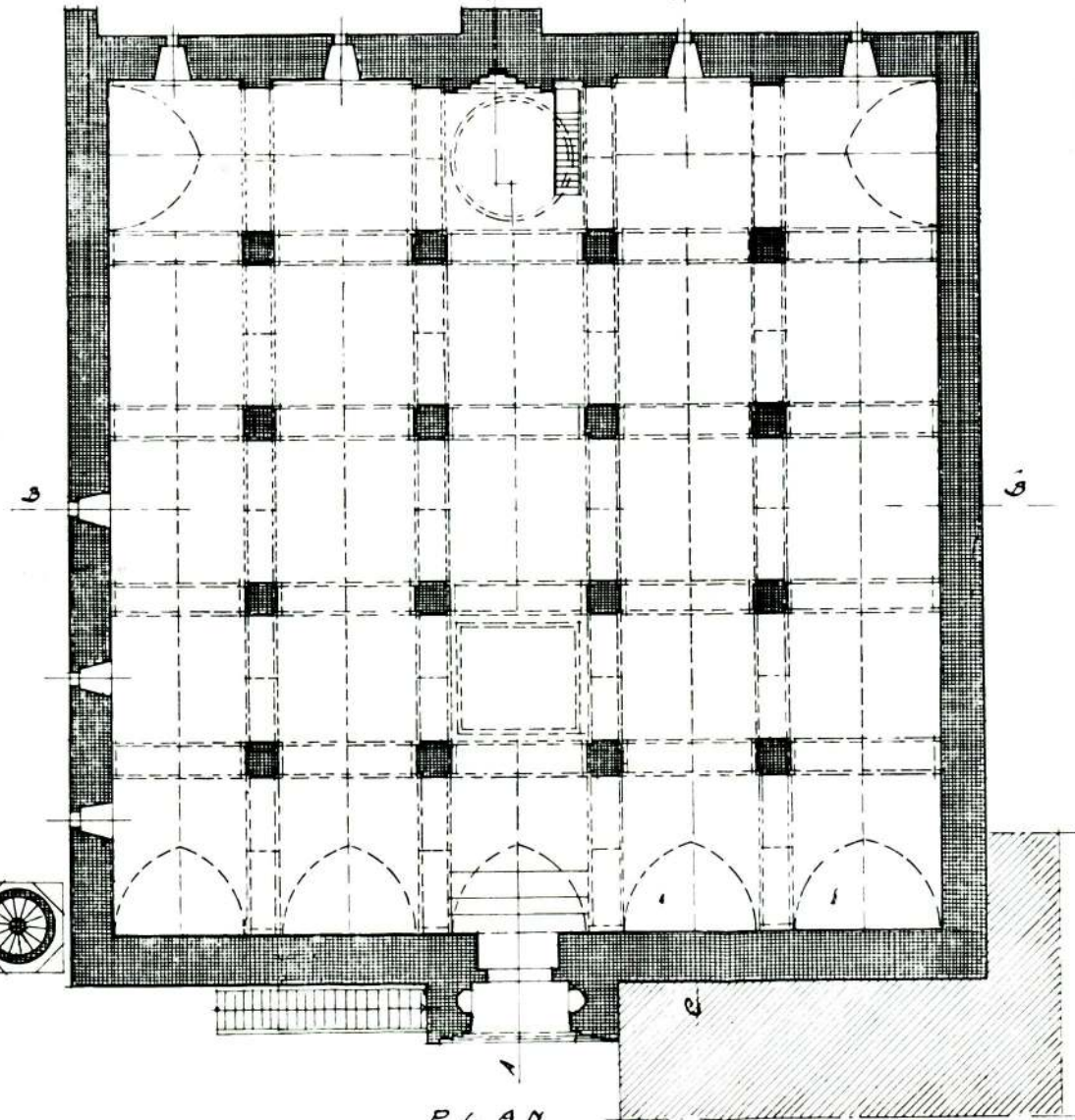
PLAN
