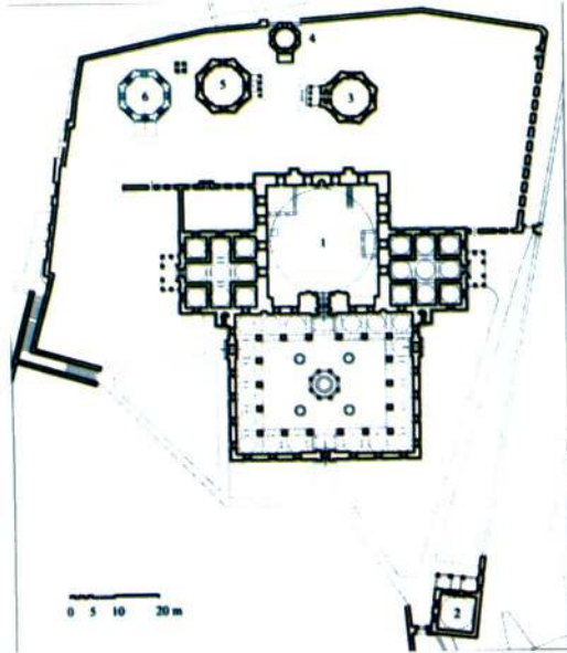
Plan 5 - İstanbul Yavuz Selim Camisi (G.Necipoglu, The Age of Sinan... , s.94).
